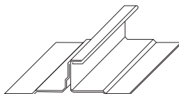
Winkelfalz Standing-seam
